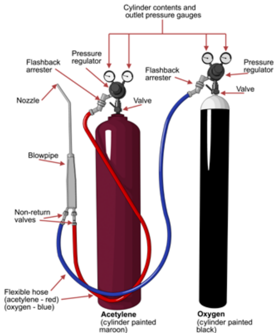
Figure 1 Typical equipment used in oxy/acetylene gas welding and similar processes (Note that cylinder valves will be operated either by a 'cylinder key' or a 'handwheel').
